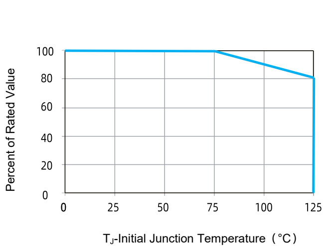
FIGURE 1 Peak Power Derating
